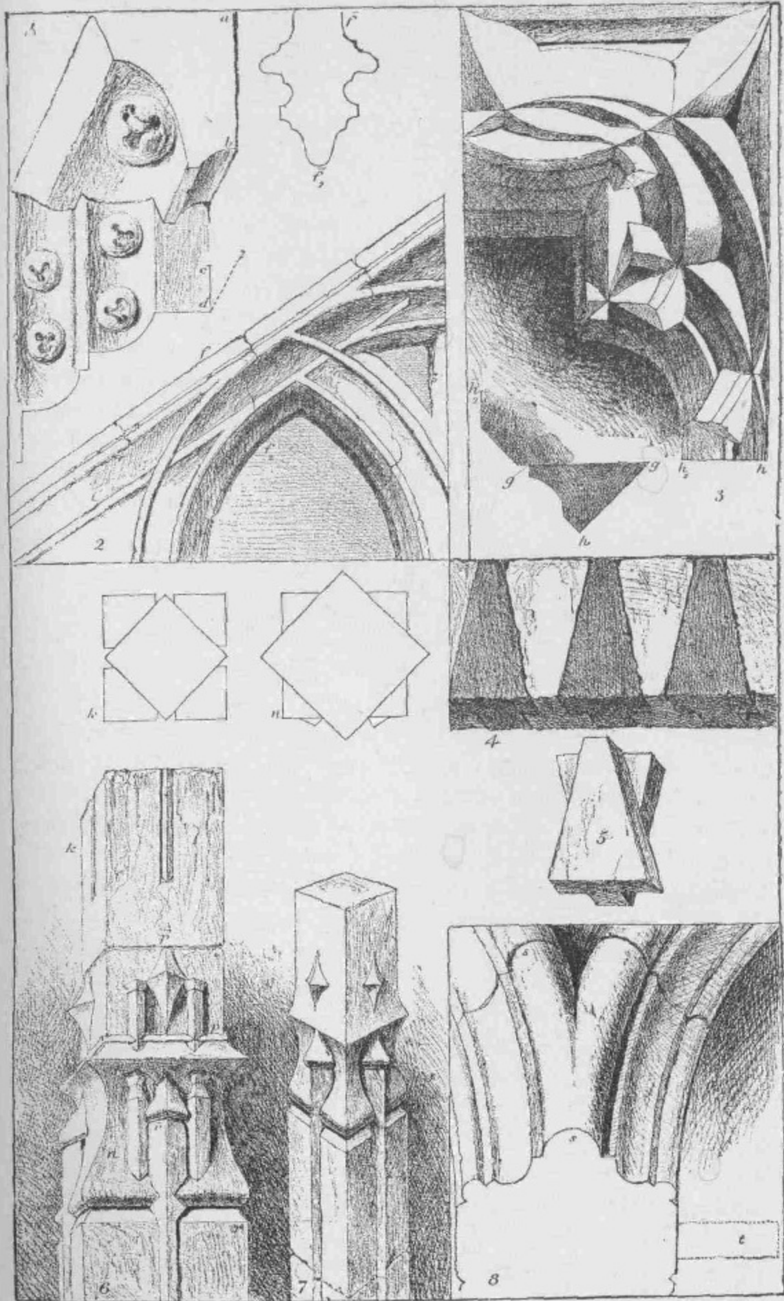
PLATE IV.—(Page 66—Vol. V.) INTERSECTIONAL MOULDINGS.
