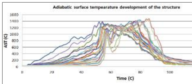
(a) Adiabatic surface temperature development of the structure
